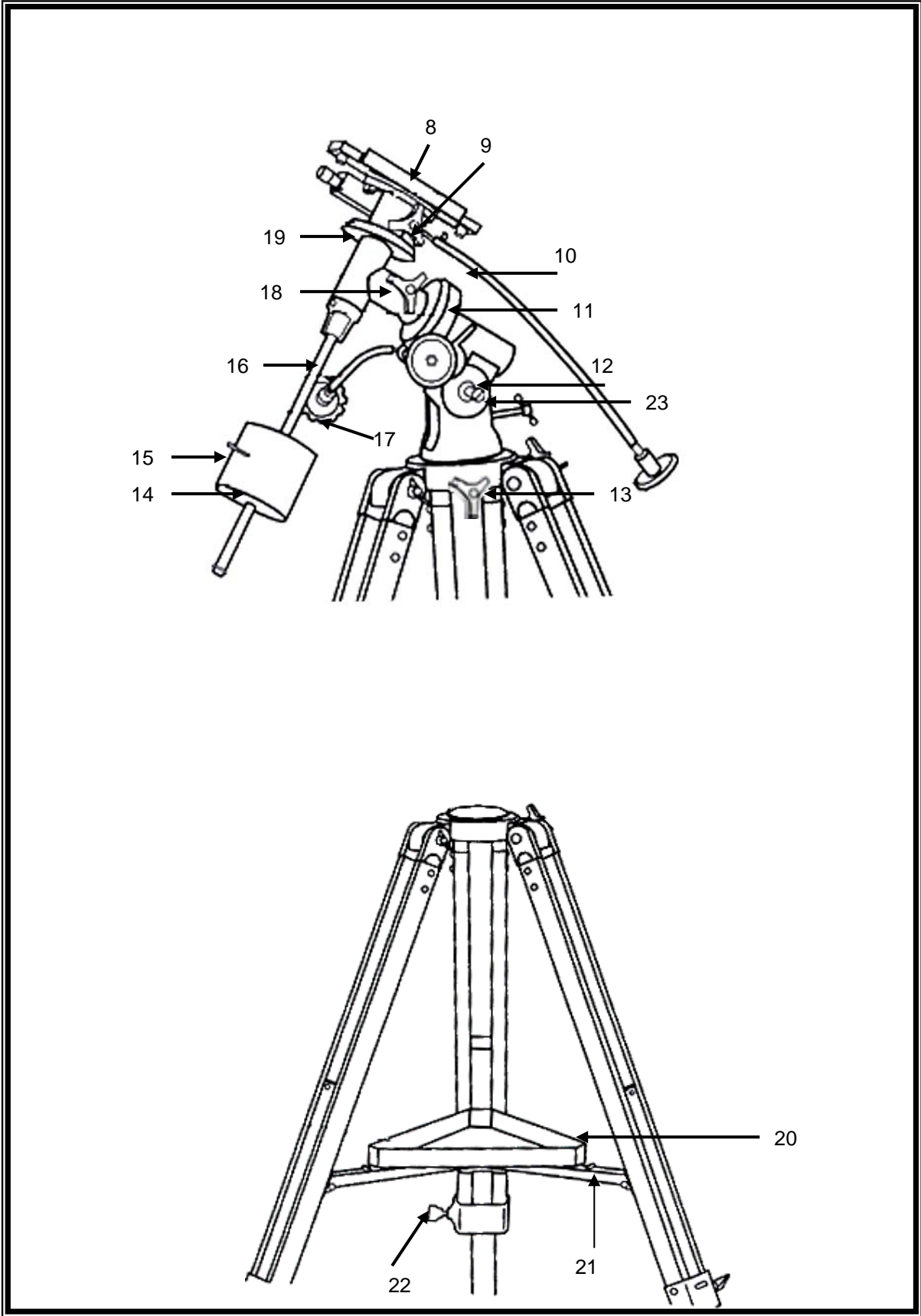
Figura 1C Montura ecuatorial
